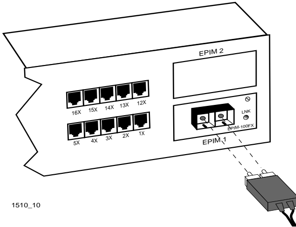
Figure A-2 EPIM-100FX
